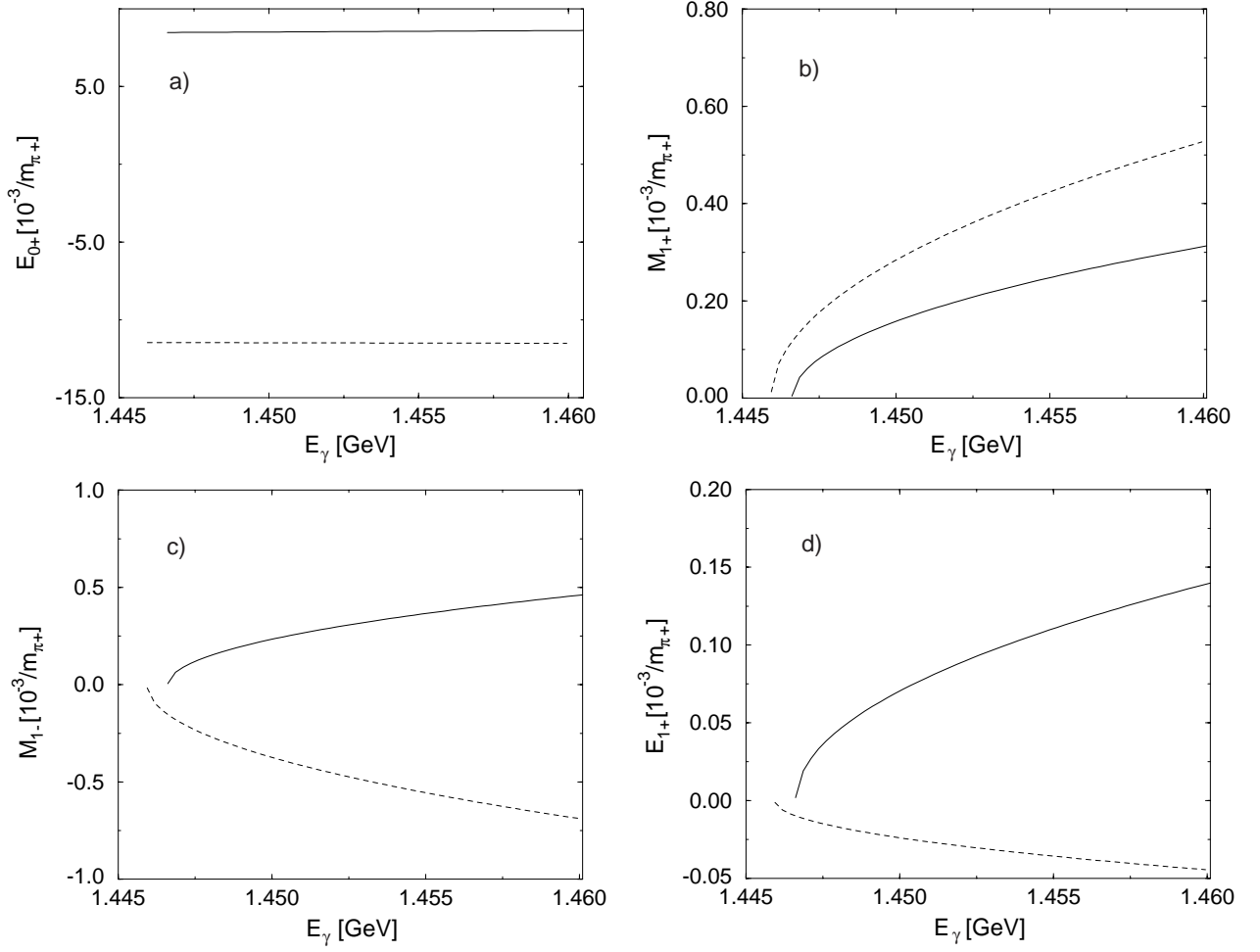
Fig. 7. Shown are the multipoles E_{0+} (a), M_{1+} (b), M_{1-} (c) and E_{1+} (d) for \eta' photoproduction off the nucleons. The full and dashed lines denote \gamma p \rightarrow p\eta' and \gamma n \rightarrow n\eta' , respectively.
