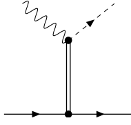
Fig. 2. Vector meson exchange. The photon is given by a wavy line. Solid and dashed lines denote nucleons and pseudoscalar mesons, respectively. The double line represents the vector meson.
