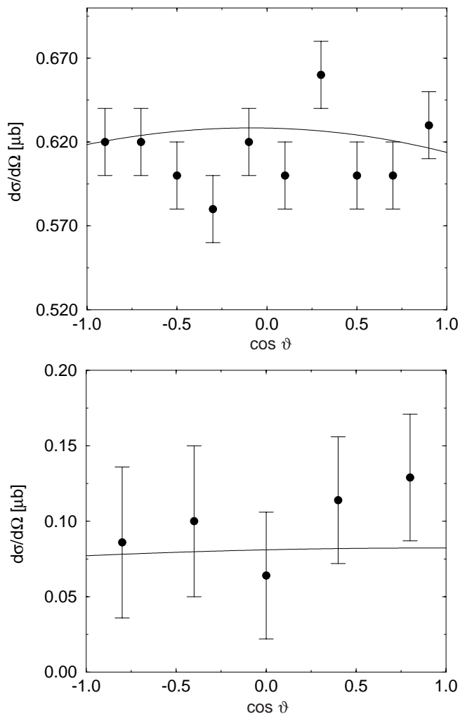
Fig. 5. a) Differential cross-section of \gamma p \rightarrow p\eta for the photon energy E_\gamma = 716 MeV which is compared with the data from [1]. b) Differential cross-section for \gamma p \rightarrow p\eta' at E_\gamma = 1.45 GeV. The data are the energy-integrated angular distributions for 1.44 \text{ GeV} < E_\gamma < 1.54 \text{ GeV} [9].
