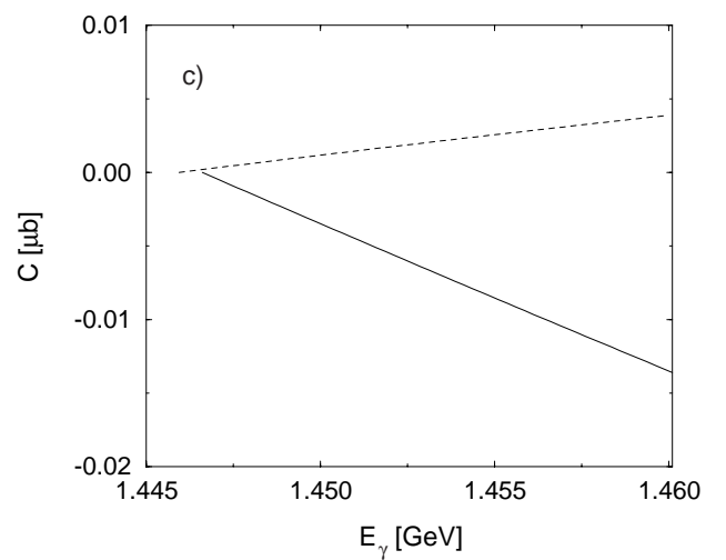
Fig. 9. Energy dependence of the coefficients A (a), B (b), C (c) from eq. (23) for \eta' photoproduction. The full and dashed lines denote \gamma p \rightarrow p\eta' and \gamma n \rightarrow n\eta' , respectively.
