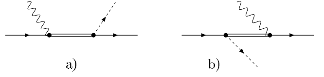
Fig. 3. Baryon resonance contributions. The photon is given by a wavy line. Solid and dashed lines denote nucleons and pseudoscalar mesons, respectively. The double line represents the baryon resonances P_{11}(1440) or S_{11}(1535) .
