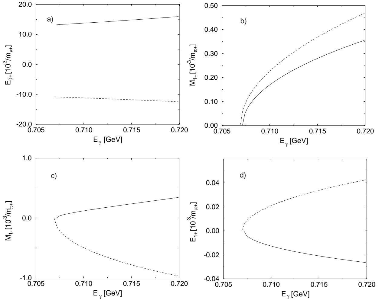
Fig. 6. Shown are the multipoles E_{0+} (a), M_{1+} (b), M_{1-} (c) and E_{1+} (d) for \eta photoproduction off the nucleons. The full and dashed lines denote \gamma p \rightarrow p\eta and \gamma n \rightarrow n\eta , respectively.
