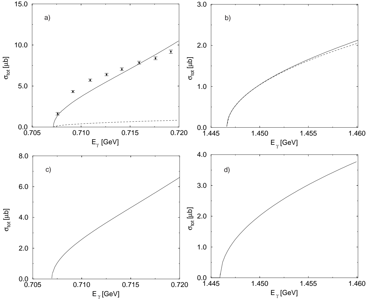
Fig. 4. Total cross-sections for \gamma p \rightarrow p\eta (a), \gamma p \rightarrow p\eta' (b), \gamma n \rightarrow n\eta (c) and \gamma n \rightarrow n\eta' (d). The dashed lines denote the contributions from the Born terms, the full lines are our results including the resonances. The reaction \gamma p \rightarrow p\eta in (a) is compared with data from [1]. We do not show data from [9] for \eta' photoproduction since the energy bins of this experiment are 100 and 200 MeV wide.
