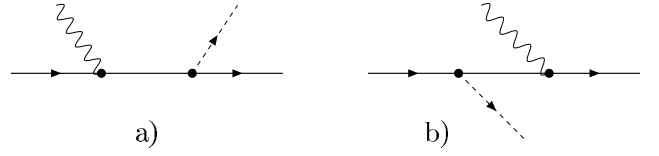
Fig. 1. Shown are the Born terms for photoproduction on the proton. The photon is given by a wavy line. Solid and dashed lines denote proton and pseudoscalar mesons, respectively.
