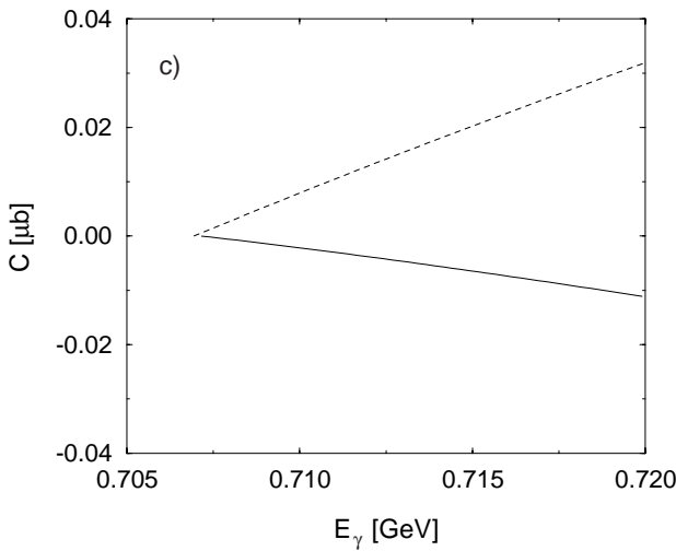
Fig. 8. Energy dependence of the coefficients A (a), B (b), C (c) from eq. (23) for \eta photoproduction. The full and dashed lines denote \gamma p \rightarrow p\eta and \gamma n \rightarrow n\eta , respectively.
